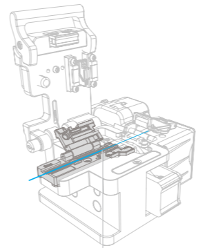
Single core optical fiber fixture
